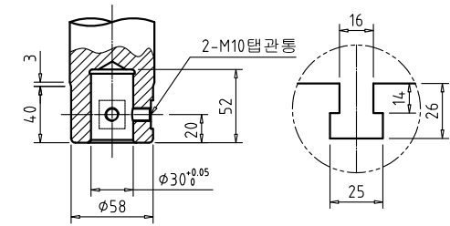
Shank Hole
